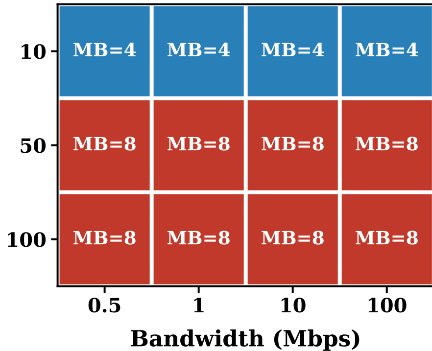
(a) Prompt = 128
