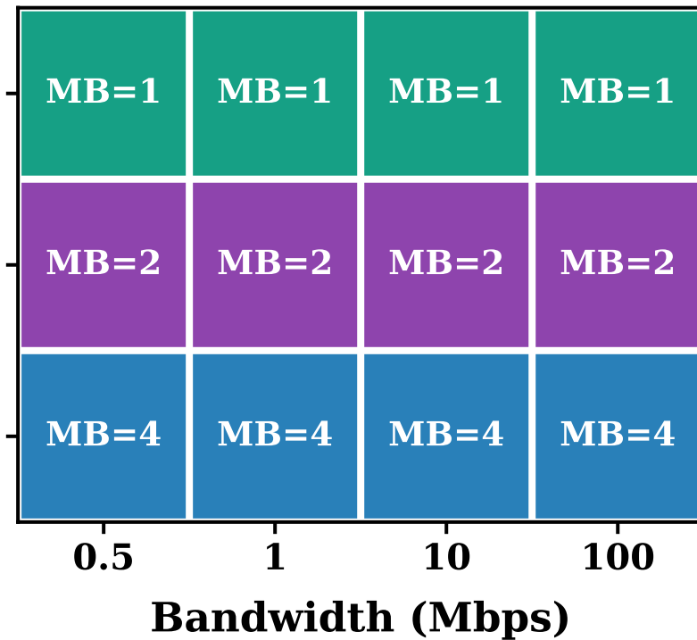
(b) Prompt = 512
