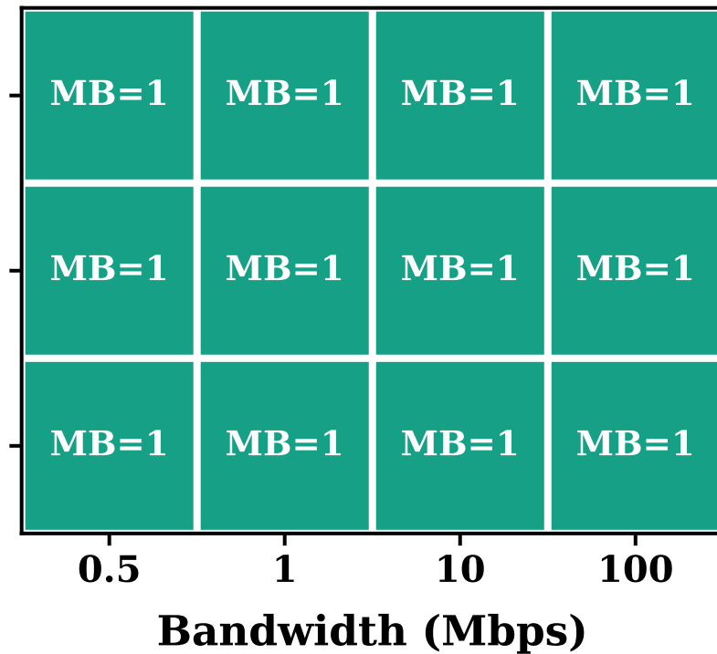
(c) Prompt = 2048
