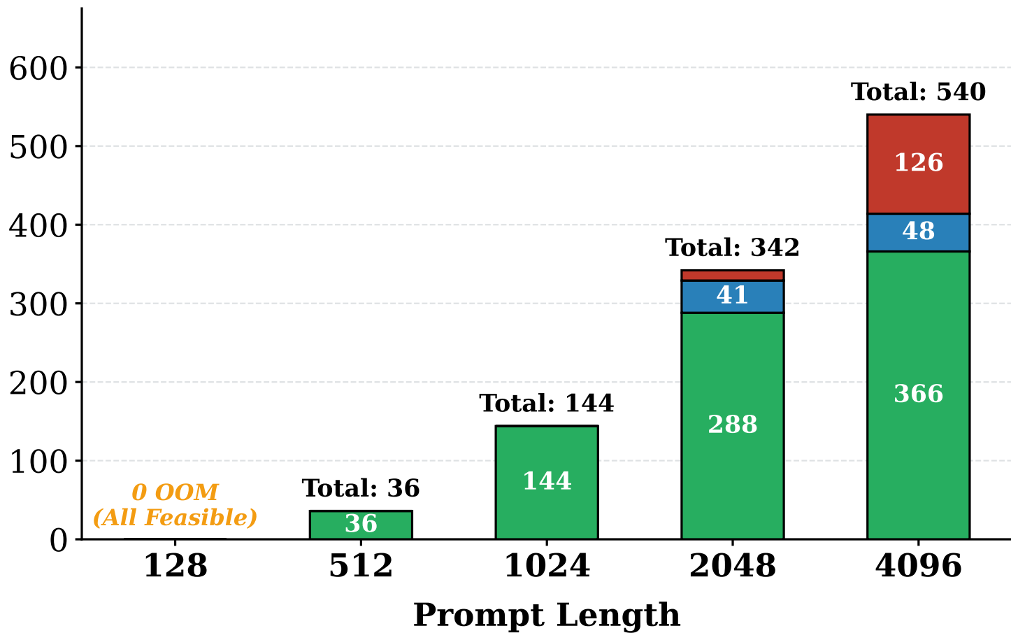
Number of Infeasible Actions (OOM)
