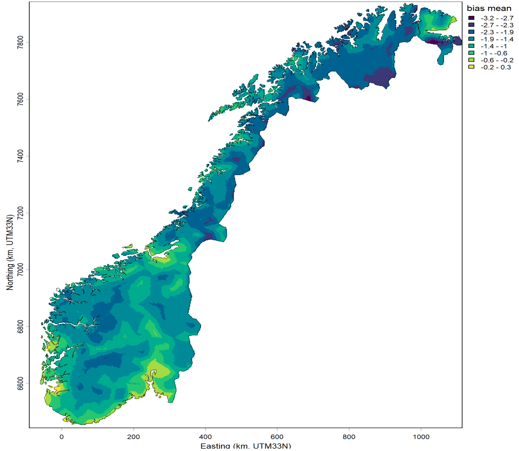
Sampling intensity (bias mean) - birds16
