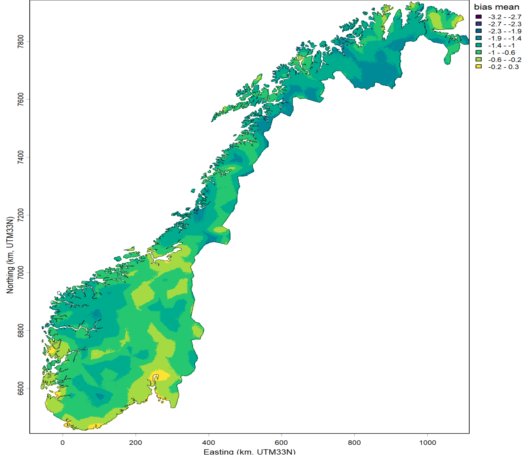
Sampling intensity (bias mean) - birds10
