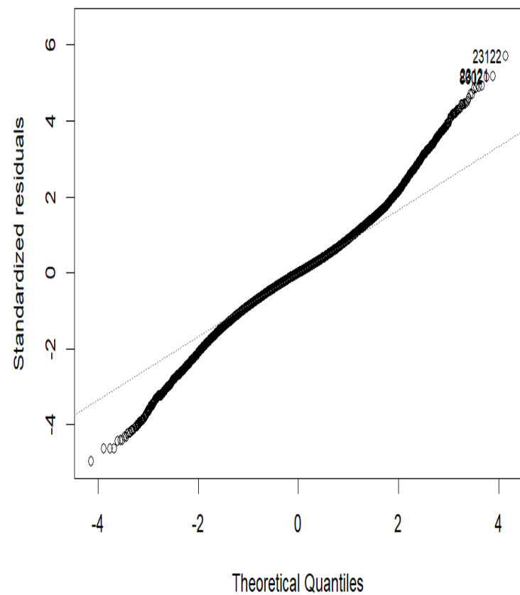
Q-Q Residuals
