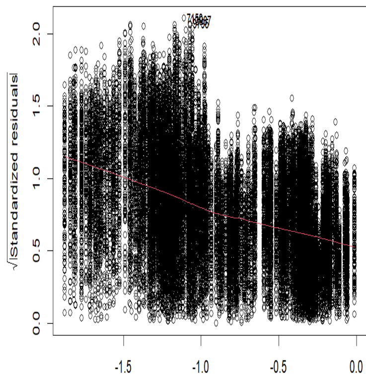
Scale-Location
