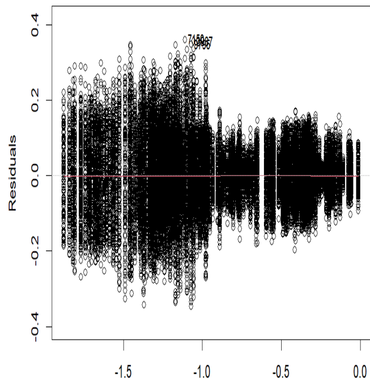
Residuals vs Fitted
