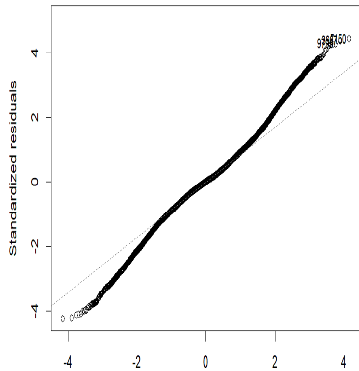
Q-Q Residuals
