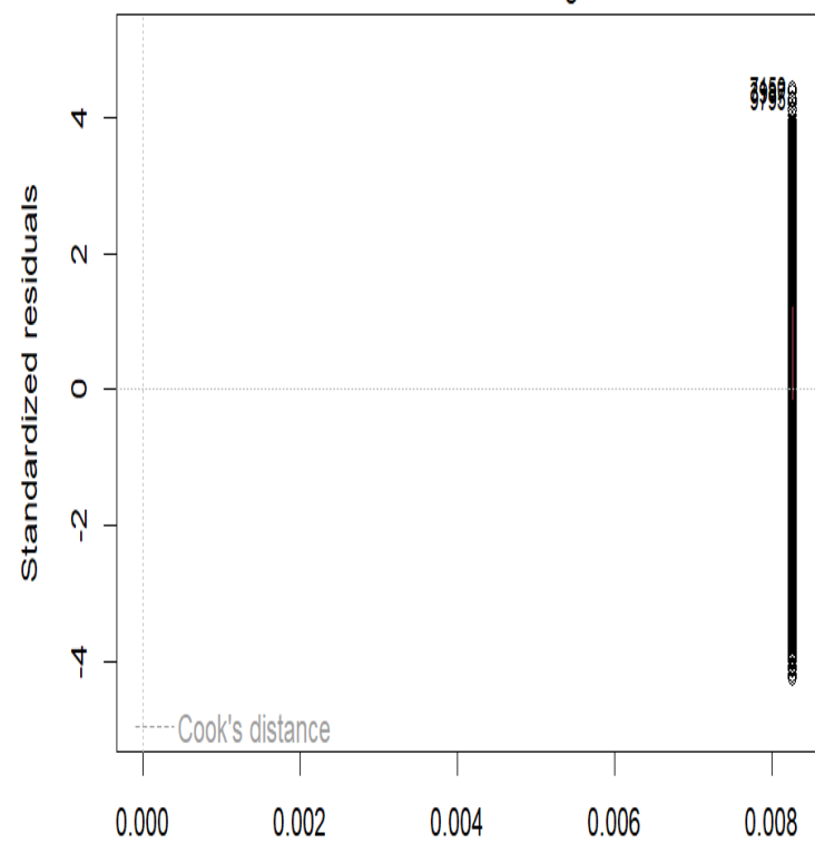
Residuals vs Leverage
