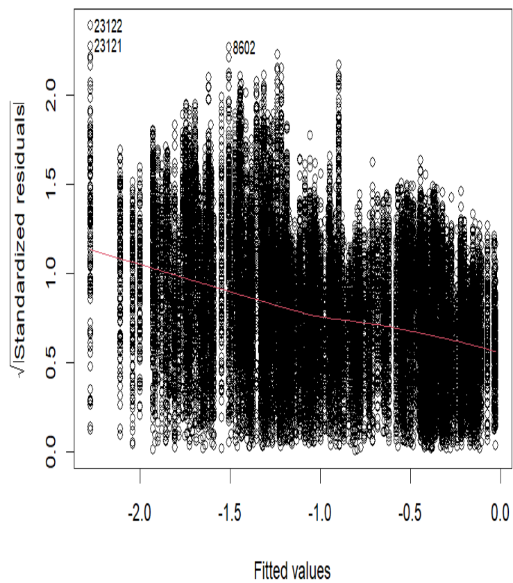
Scale-Location
