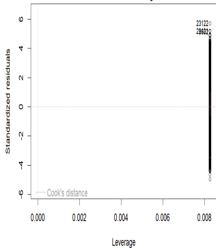
Residuals vs Leverage
