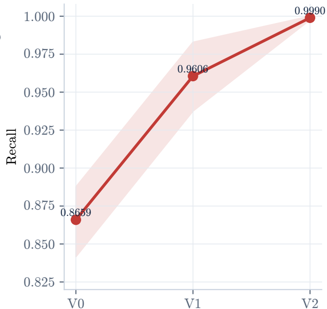
Recall
