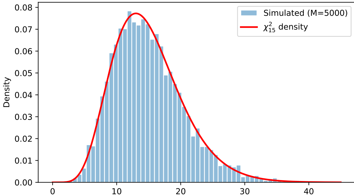
Part 1.1: W = \text{sum of 15 squared } N(0,1)
