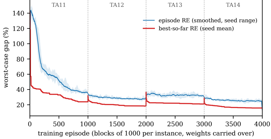
Fig. 2 Training dynamics of the deployed arm: worst-case gap to the instance bound of the sampled training episodes (smoothed over 25 episodes; the band spans the seeds) and of the best schedule found so far, over the four training blocks TA11–TA14. The training logs record the worst-case makespan, the quantity the reward optimizes, so the axis is not the midpoint RE of Eq. (4).
