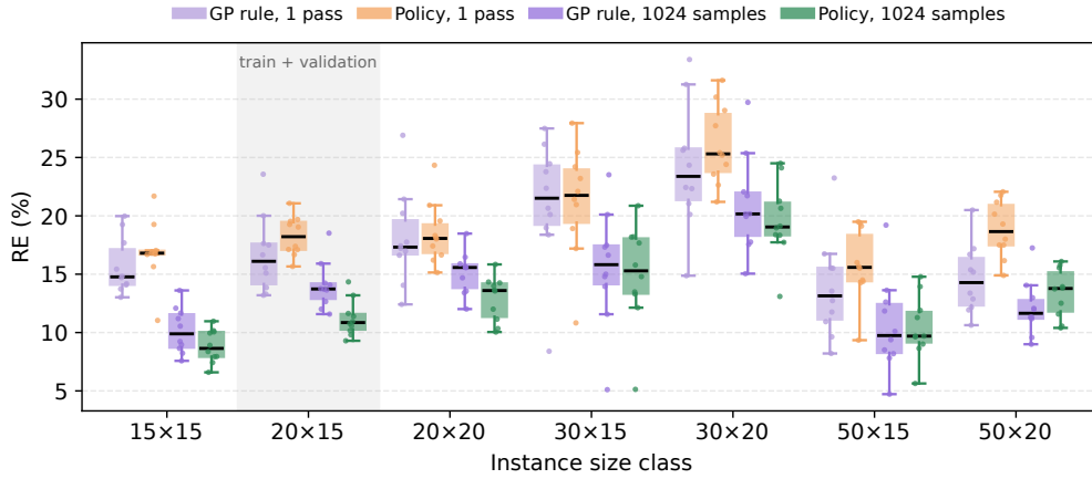
Fig. 4 RE by size class over the 70 interval Taillard instances, the two learners paired at one pass and at 1024 samples. Boxes span the quartiles with whiskers at 1.5 IQR; every instance is overlaid as a point. The shaded 20 \times 15 class holds the training and validation instances.
