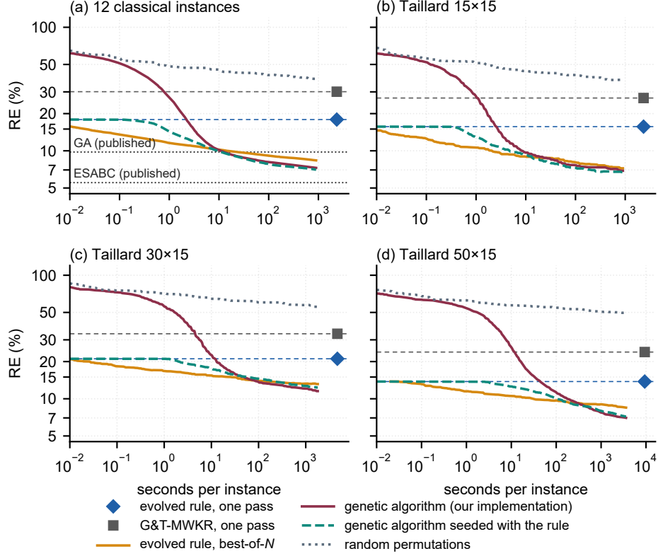
Figure 4: RE against seconds per instance on the 12 classical instances (a) and on three Taillard classes with 15 machines, 15 \times 15 (b), 30 \times 15 (c) and 50 \times 15 (d). Each curve is the mean over the instances of the mean over runs of the RE of the incumbent solution, with 30 runs per instance in (a) and 3 in (b)–(d). The single-pass methods are horizontal reference lines, marked at their right end; in (a) the dotted lines are the results published for the genetic algorithm and ESABC.
