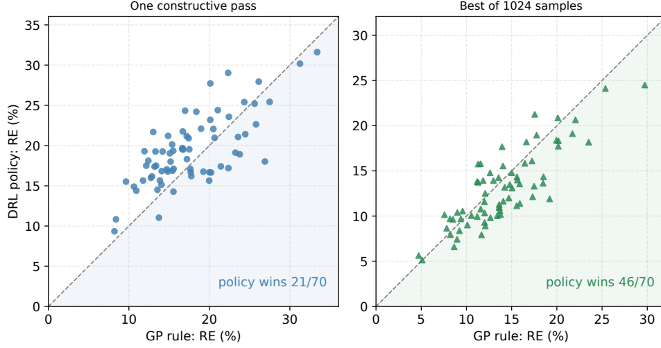
Fig. 4 The DRL policy against the GP rule (?) at matched inference budgets, one point per instance over the 70 interval Taillard instances. Points below the diagonal are instances where the policy wins. Left: one constructive pass each. Right: 1024 samples each, the rule randomized with \epsilon -greedy dispatching.
