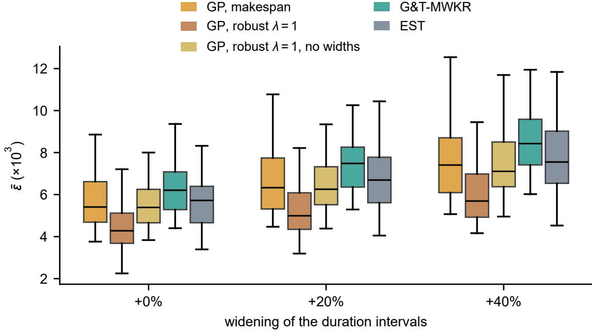
Figure S1: Per-instance \bar{\varepsilon} by method at nominal interval widths and widened by +20% and +40%; the robust \lambda=1 entries are the rules of Table 8.
