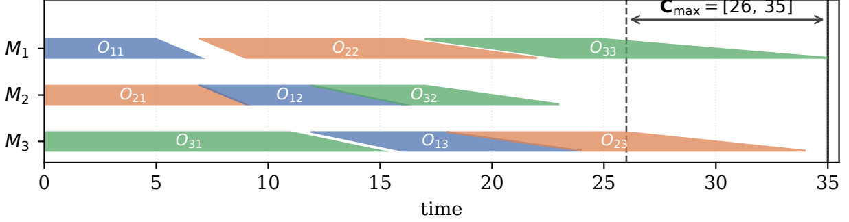
Figure 1: A processing order on a 3 \times 3 interval instance does not fix one schedule but a family of them. Each operation is a single shape whose upper edge runs from s^L to e^L and whose lower edge runs from s^U to e^U : the upper edge is the schedule that results when every duration takes its lower endpoint, the lower edge the one that results at the upper endpoint, and the two sloped sides are the slack in the start and in the completion. Operation O_{jk} is the k -th operation of job j , and consecutive operations on a machine share a side. The interval makespan of Eq. (2) is [26, 35] , whose two endpoints come from different jobs: job 2 finishes in [26, 34] and job 3 in [25, 35] , so neither endpoint of \mathbf{C}_{\max} is the completion of a single job.
