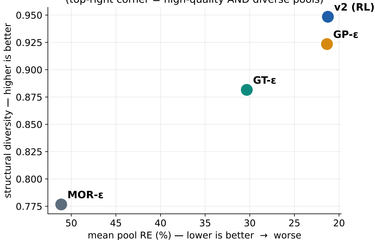
Seed generators: quality vs. diversity (top-right corner = high-quality AND diverse pools)
