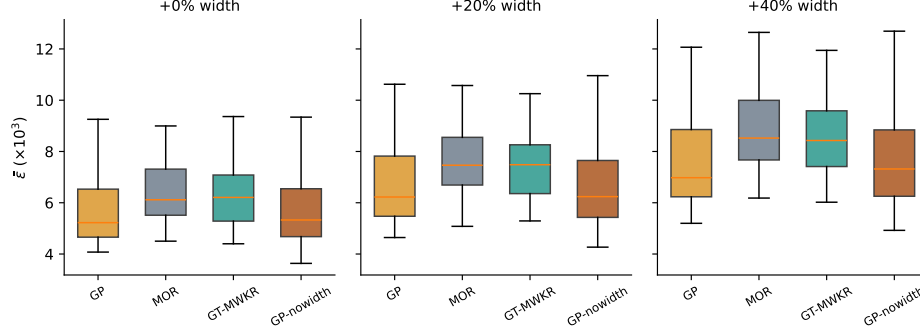
Figure 8: Per-instance \bar{\epsilon} robustness by method at each uncertainty level (lower is better). The evolved rule’s robustness advantage over the constructive baselines grows with interval width.
