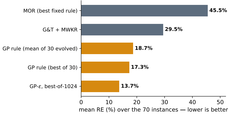
Figure 4: Constructive-method ladder on the 70 interval Taillard instances. Bars are single-solution methods except where noted.
