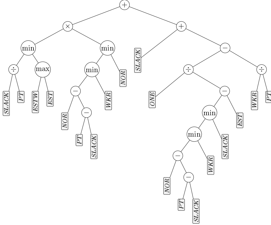
Figure 2: The best evolved rule of the campaign (seed 27), which attains 17.3% RE over the 70 instances. Circles are functions and shaded boxes the interval-aware terminals of Table 1; the operation with the lowest value of the expression is dispatched. The tree is shown exactly as evolved, without algebraic simplification.
