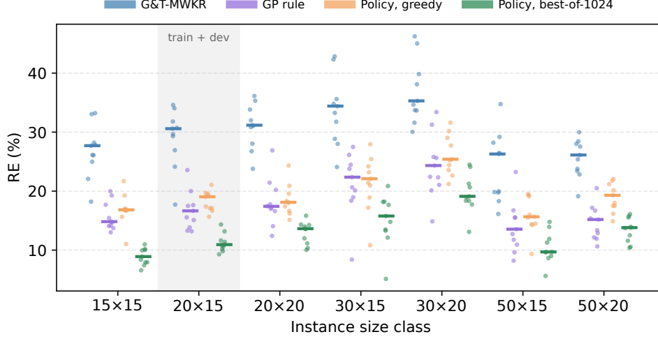
Fig. 4 Per-instance RE by size class over the 70 interval Taillard instances: every instance is a point, bars mark class medians. The 20 \times 15 class is shaded because it holds the four training and six development instances; the other six classes were touched by neither.
