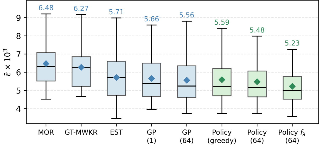
Figure 11: Executional robustness by method: \bar{\varepsilon} \times 10^3 over the seventy benchmark instances; lower is a more faithful prediction. Boxes span the quartiles with whiskers at 1.5 IQR, and diamonds mark the means quoted in the text; the number in parentheses is the inference budget in constructed schedules.
