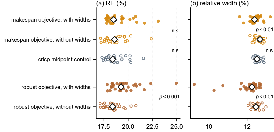
Figure 8: Ablations of the interval machinery: the 30 evolved rules of each arm, each averaged over the 70 instances, in RE (a) and in the relative width of the predicted makespan interval (b). Diamonds mark the median of each arm, and the label between two arms gives their Mann–Whitney test.
