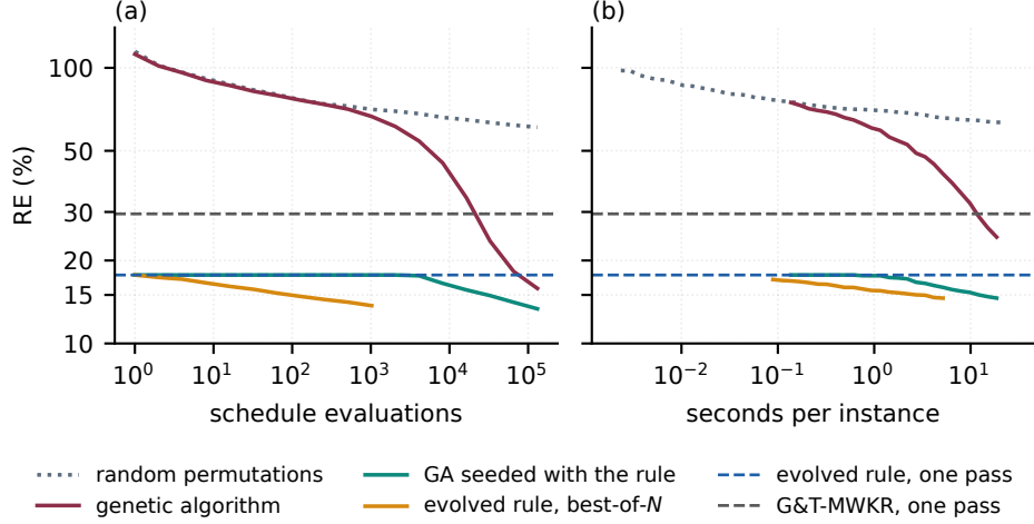
Figure 4: RE over the 70 instances against budget, measured in schedules constructed (a) and in seconds of this implementation (b). No curve is drawn beyond the budget at which it was measured.
