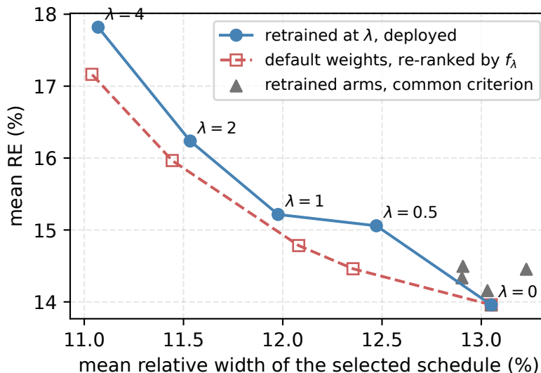
Figure 10: Mean relative width of the selected schedule against its mean RE, over the 60 (instance, seed) pools of each arm’s common rollout deposit, under three selection regimes.
