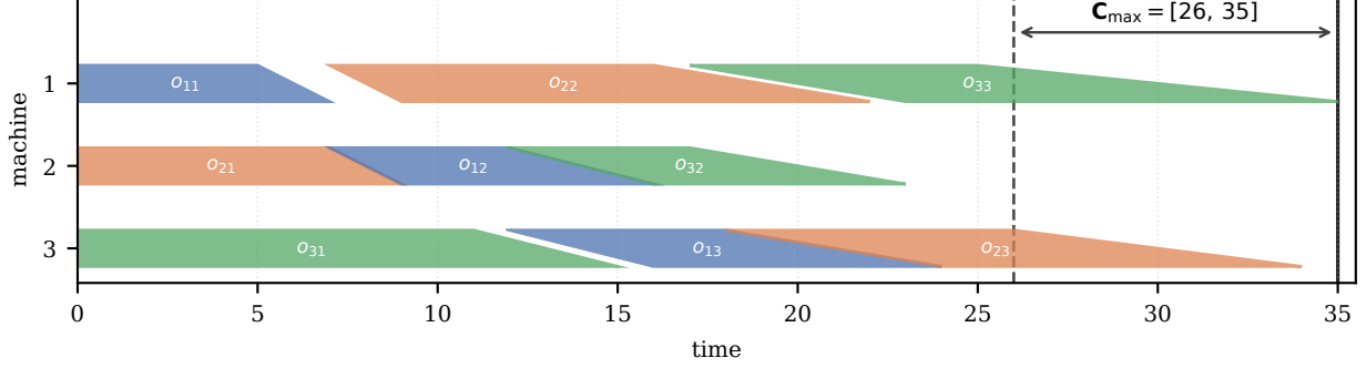
Figure 1: A processing order on a 3 \times 3 interval instance and the family of schedules it induces.
