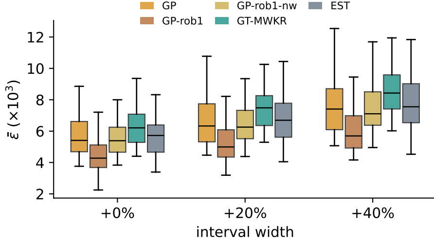
Figure 8: Per-instance \bar{\epsilon} by method at each uncertainty level (lower is better). GP-rob1 is the narrowest rule of the robust \lambda=1 arm and GP-rob1-nw its counterpart evolved without the width terminals.
