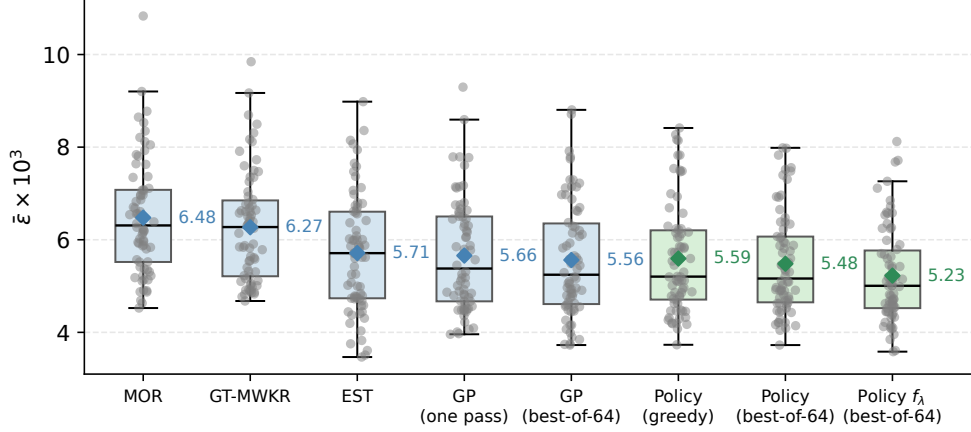
Fig. 10 Executional robustness by method: \bar{\epsilon} \times 10^3 over the seventy benchmark instances; lower is a more faithful prediction. Boxes span the quartiles with whiskers at 1.5 IQR, every instance is overlaid as a point, and diamonds mark the means quoted in the text.
