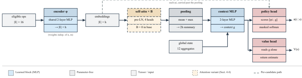
Fig. 1 The size-invariant network. Every eligible operation is embedded by the same MLP \phi ; mean and max pooling collapse the variable-size candidate set into fixed-size summaries that, joined with the global features, form the context g . Because pooling discards candidate identity, each embedding \phi_i is also carried past it (dashed grey path) so the policy head can score [\phi_i; g] pairs; the value head reads g alone. The dashed block marks where the self-attention variant of Section 4.4 inserts, with B=0 recovering the base model. No dimension depends on the numbers of jobs or machines.
