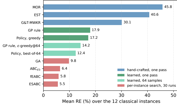
Fig. 3 Mean RE over the 12 classical interval instances, grouped by the inference budget each method is given. The two learned methods are shown at both budgets, since comparing one against the other across budgets would confound the method with what it is allowed to spend: at one pass they are indistinguishable, and the policy’s lead appears only once both may sample.
