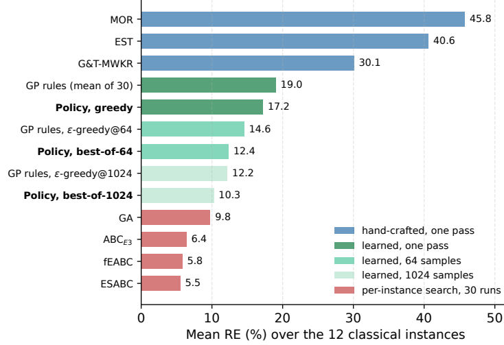
Fig. 5 Mean RE over the 12 classical interval instances, grouped by the inference budget each method is given. Both learned entries are means over independent runs.
