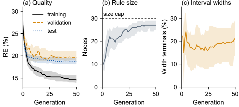
Figure 2: The best rule of each generation over the 30 independent evolutions: (a) its RE on the training, validation and test instances, (b) its size in nodes, and (c) the share of interval-width terminals among its leaves. Lines are medians, means in (c); shaded bands are interquartile ranges.
