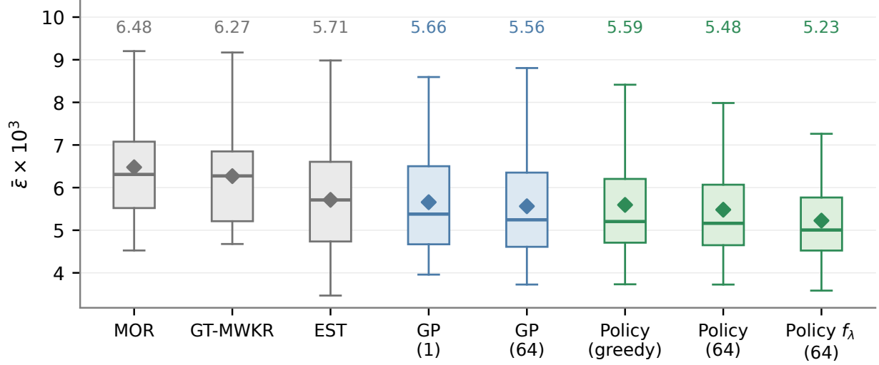
Figure 11: Executional robustness by method: \bar{\varepsilon} \times 10^3 over the seventy benchmark instances; lower is a more faithful prediction. Boxes span the quartiles with whiskers at 1.5 IQR, and diamonds mark the means quoted in the text; the number in parentheses is the inference budget in constructed schedules.
