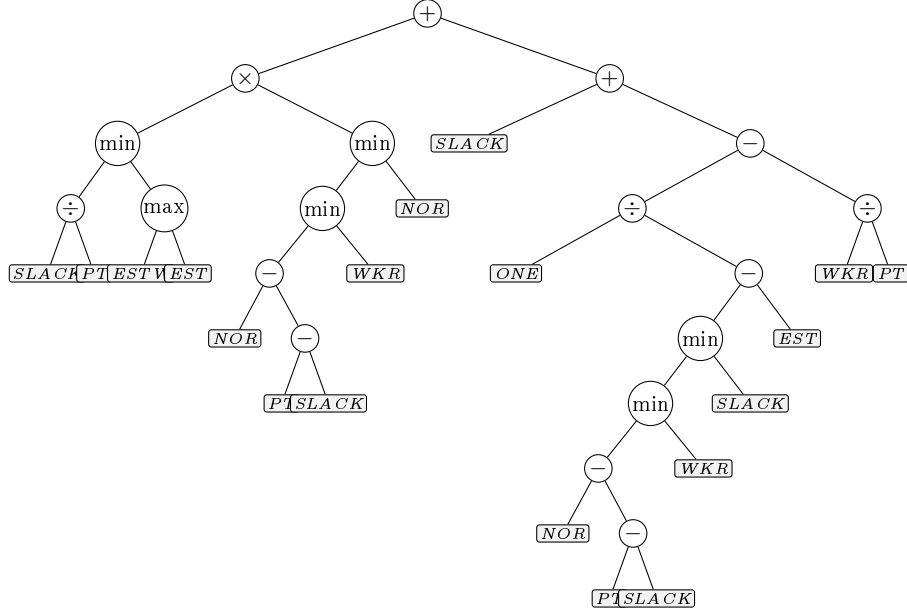
Figure 2: The best evolved rule of the campaign (seed 27), which attains 17.3% RE over the 70 instances. Circles are functions and shaded boxes the interval-aware terminals of Table 1; the operation with the lowest value of the expression is dispatched. The tree is shown exactly as evolved, without algebraic simplification.
