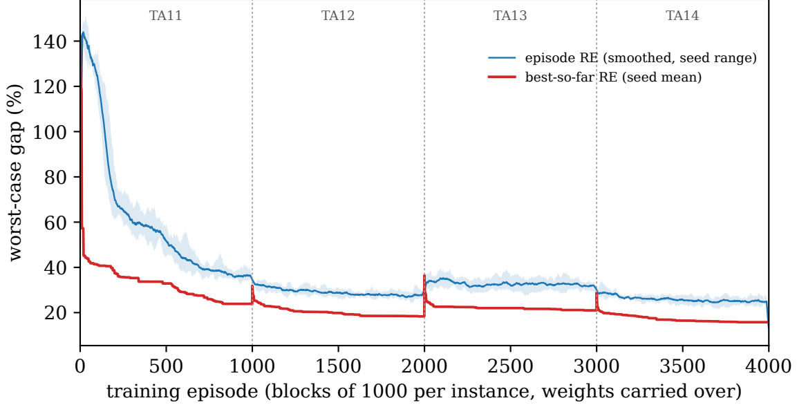
Figure 4: Training dynamics of the deployed arm: worst-case gap to the instance bound of the sampled training episodes (smoothed over 25 episodes; the band spans the best and worst seed) and of the best schedule found so far, over the four training blocks TA11–TA14. The training logs record the worst-case makespan, the quantity the reward optimizes, so the axis is not the midpoint RE of Eq. (4).
