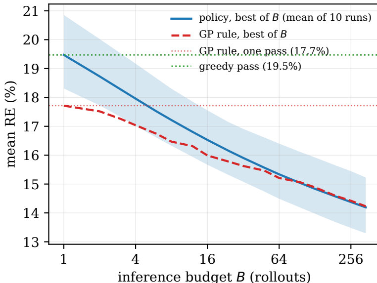
Figure 7: RE against the inference budget B on a base-2 logarithmic axis, for both learners under the same decoder: the schedule each retains from its deterministic pass plus B - 1 samples, kept by the criterion of Eq. (3) and averaged over the 70 instances. The policy curve is the mean over the ten training runs and the band spans the best and worst of them; the dotted line marks the rule’s single deterministic pass.
