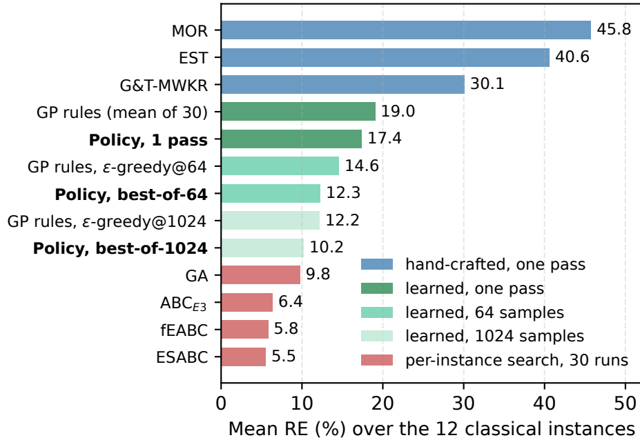
Figure 5: Mean RE over the 12 classical interval instances, grouped by the inference budget each method is given. Both learned entries are means over the thirty independent runs of their family.
