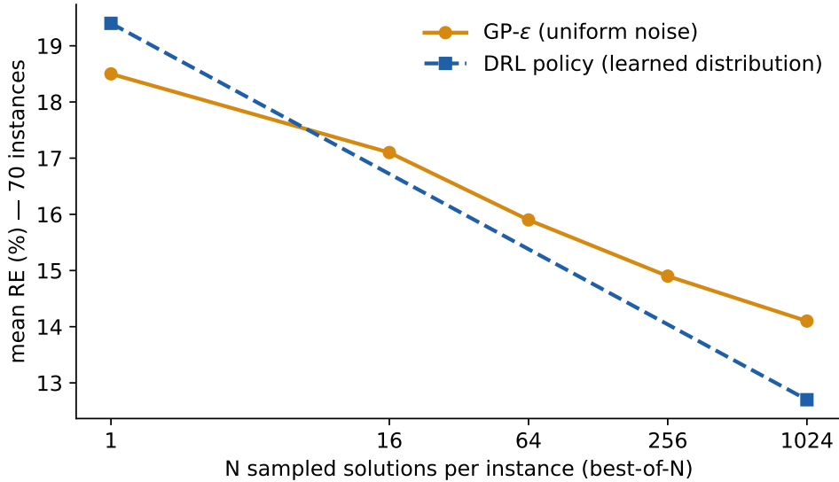
Figure 3: Best-of- N curves at matched inference budgets: the evolved rule with uniform \epsilon -randomization versus the companion DRL policy sampling from its learned distribution.
