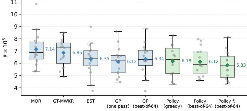
Fig. 9 Executional robustness by method: \bar{\varepsilon} \times 10^3 over the fifteen evaluation instances; lower is a more faithful prediction. Boxes span the quartiles with whiskers at 1.5 IQR, every instance is overlaid as a point, and diamonds mark the means quoted in the text.
