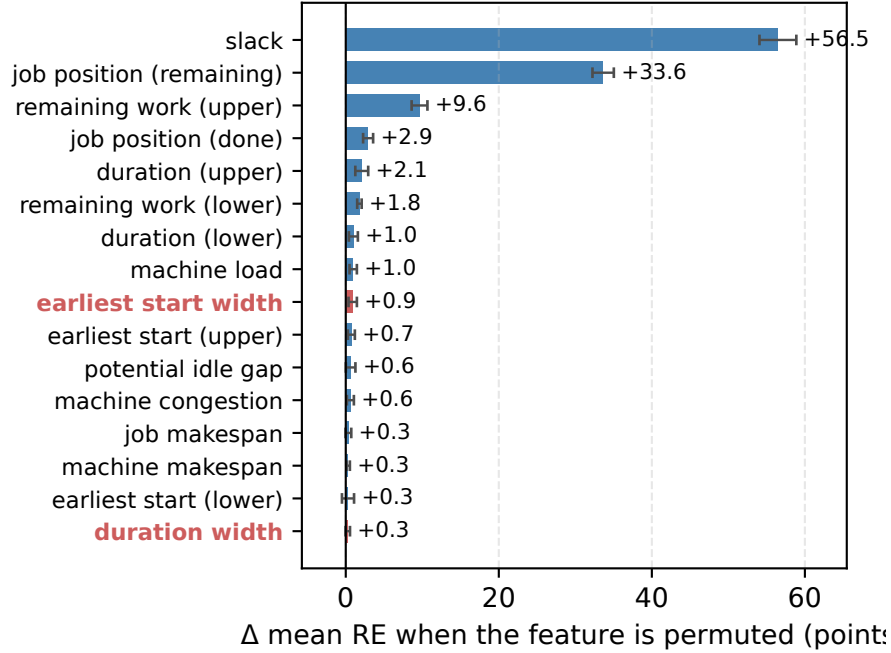
Figure 6: Permutation importance of the 16 operation features, as the change in mean validation-set RE. Bars are the mean of five independent permutation draws and whiskers their standard deviation; the two interval-width features are highlighted.
