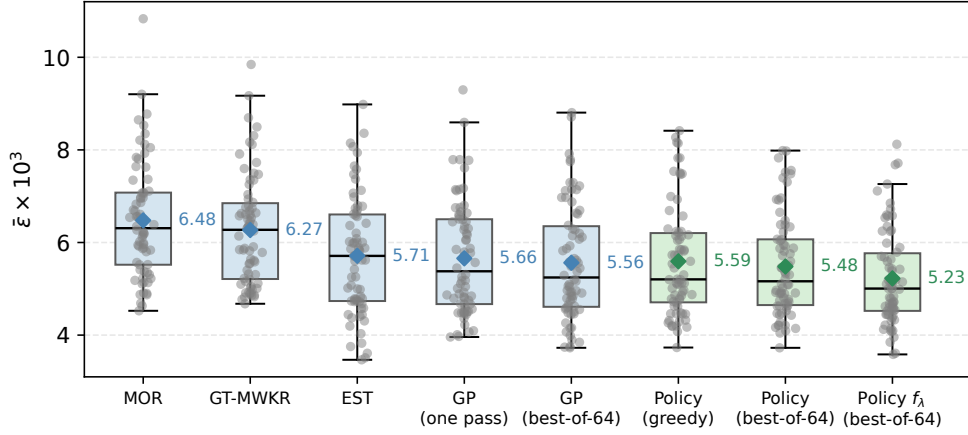
Fig. 9 Executorial robustness by method: \bar{\varepsilon} \times 10^3 over the seventy benchmark instances; lower is a more faithful prediction. Boxes span the quartiles with whiskers at 1.5 IQR, every instance is overlaid as a point, and diamonds mark the means quoted in the text.
