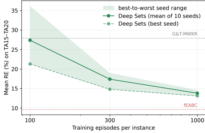
Fig. 3 Mean RE on the development set against the training budget, the episodes spent once per instance before deployment, on a logarithmic axis and over ten training runs. The band spans the best and worst of them; the dotted lines are G&T-MWKR and fEABC on the same six instances.
