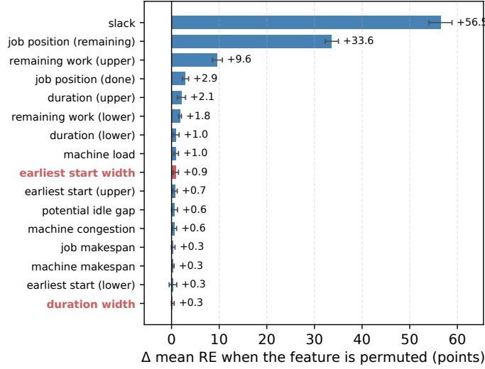
Fig. 7 Permutation importance of the 16 operation features: change in mean development-set RE when the feature’s column is shuffled across the eligible operations at every decision (greedy rollouts, three seeds; intact baseline 18.2%). Bars are the mean of five independent permutation draws and whiskers their standard deviation. The two interval-width features are highlighted.
