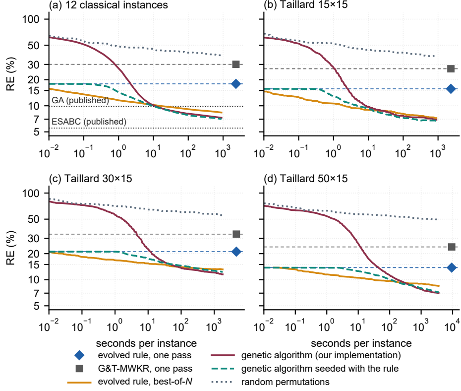
Figure 4: Mean RE of the best schedule found, over runs and instances, against seconds per instance on the 12 classical instances (a) and on three Taillard classes with 15 machines, 15 \times 15 (b), 30 \times 15 (c) and 50 \times 15 (d).
