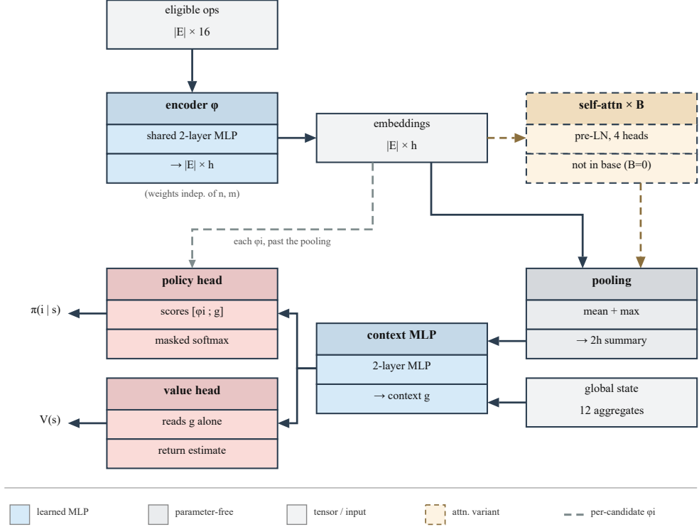
Fig. 1 The size-invariant network; solid edges are the base model’s data path. Every eligible operation is embedded by the same MLP \phi ; mean and max pooling collapse the variable-size candidate set into fixed-size summaries that, joined with the global features, form the context g . Because pooling discards candidate identity, each embedding \phi_i is also carried past it (grey dashed path) so the policy head can score [\phi_i; g] pairs; the value head reads g alone. The dashed detour is the self-attention variant of Section 4.4: it is not part of the base model ( B=0 ), and Section 7.3 finds it does not pay for itself. No dimension depends on the numbers of jobs or machines.
