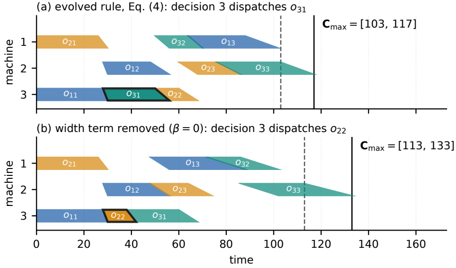
Figure 6: The worked example scheduled by the evolved rule and by the same rule without the width term. The outlined operation is the one that separates the two traces.
