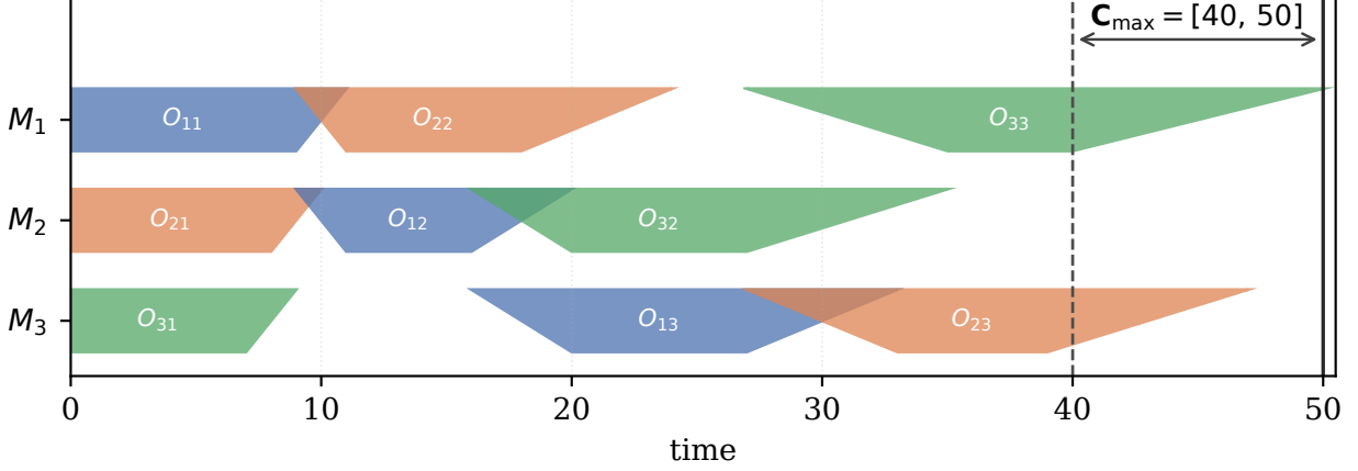
Figure 1: A processing order on a 3 \times 3 interval instance does not fix one schedule but a family of them. Each operation is a single shape whose left edge rises from s^L to s^U and whose right edge falls from e^L to e^U : the flat top is the span in which the operation holds its machine under every realization, and the sloped edges are the slack in its start and in its completion. Operation O_{jk} is the k -th operation of job j . Consecutive operations on a machine interlock along the edges they share, and the interval makespan of Eq. (2) is [40, 50] .
