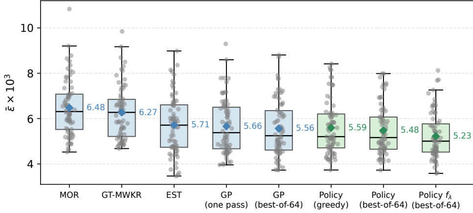
Fig. 10 Executional robustness by method: \bar{\varepsilon} \times 10^3 over the seventy benchmark instances; lower is a more faithful prediction. Boxes span the quartiles with whiskers at 1.5 IQR, every instance is overlaid as a point, and diamonds mark the means quoted in the text.
