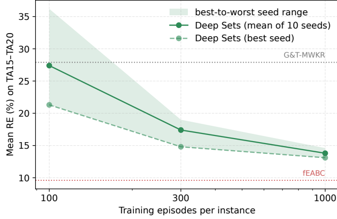
Fig. 3 Mean RE on the six validation instances TA15–TA20 ( 20 \times 15 ) against the training budget, the episodes spent once per instance before deployment, on a logarithmic axis and over ten training runs. The band spans the best and worst of them; the dotted lines are G&T-MWKR and fEABC on the same six instances.
