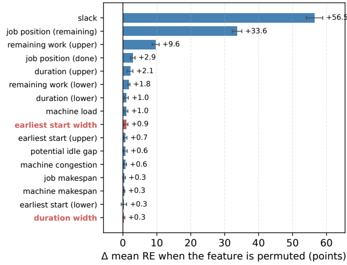
Fig. 7 Permutation importance of the 16 operation features: change in mean validation-set RE when the feature’s column is shuffled across the eligible operations at every decision (greedy rollouts, three seeds; intact baseline 18.2%). Bars are the mean of five independent permutation draws and whiskers their standard deviation. The two interval-width features are highlighted.
