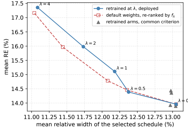
Fig. 8 Mean relative width of the selected schedule against its mean RE, over the 60 (instance, seed) pools of each arm’s common rollout deposit, under three selection regimes.
