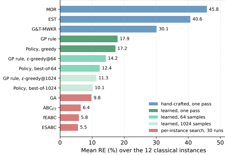
Fig. 3 Mean RE over the 12 classical interval instances, grouped by the inference budget each method is given. The two learned methods are shown at both budgets, since comparing one against the other across budgets would confound the method with what it is allowed to spend: at one pass they are indistinguishable, and the policy’s lead appears only once both may sample.
