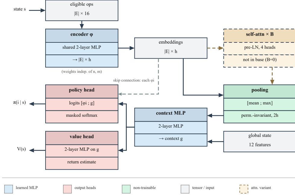
Fig. 1 The size-invariant policy/value network. Solid edges are the base model’s data path; the grey dashed edge is the per-candidate skip connection; the dashed detour is the self-attention variant of Section 4.4, not part of the base model ( B=0 ).
