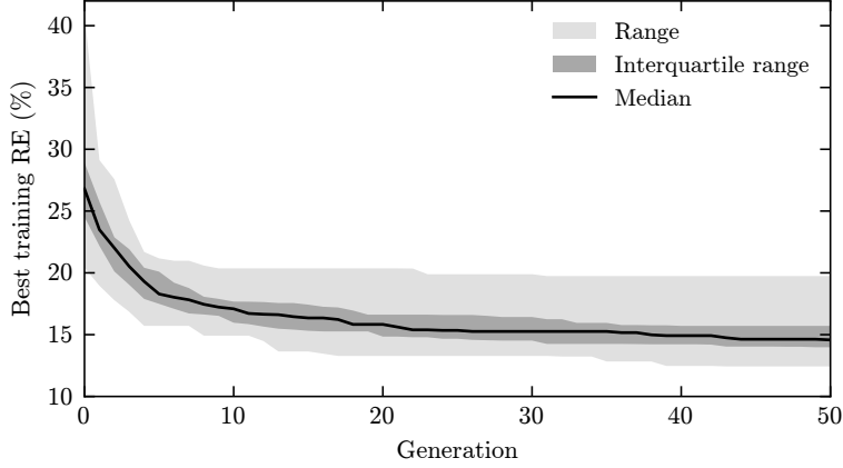
Figure 2: Best training RE per generation over the 30 independent evolutions: median, interquartile range and range.
