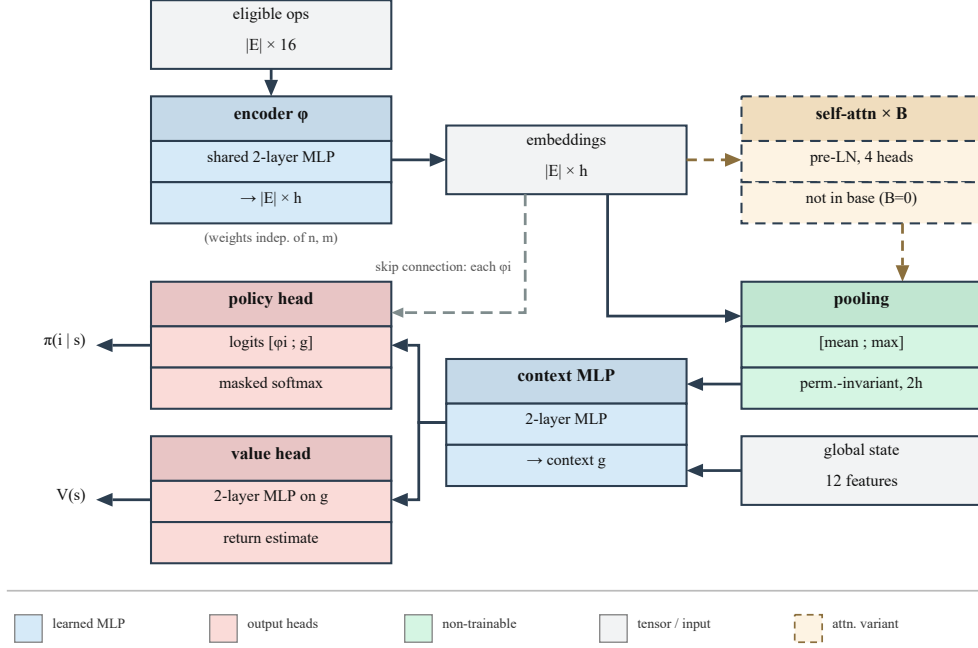
Fig. 1 The size-invariant network; solid edges are the base model’s data path. Every eligible operation is embedded by the same MLP \phi ; mean and max pooling collapse the variable-size candidate set into fixed-size summaries that, joined with the global features, form the context g . Because pooling discards candidate identity, each embedding \phi_i is also carried past it (grey dashed skip connection) so the policy head can score [\phi_i; g] pairs; the value head reads g alone. The dashed detour is the self-attention variant of Section 4.4: it is not part of the base model ( B=0 ), and Section 7.3 finds it does not pay for itself. No dimension depends on the numbers of jobs or machines.
