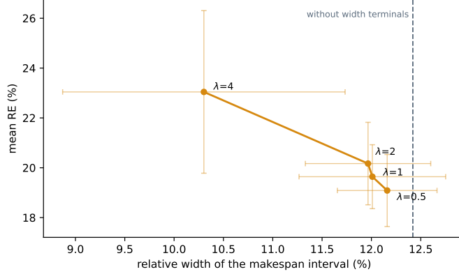
Figure 5: Quality–predictability frontier traced by the weight \lambda of the robust fitness, Eq. (13). Rules evolved with the interval-width terminals (mean \pm sd over independent evolutions, each evaluated on the 70 instances); the dashed line marks the arm evolved without them, which cannot narrow the interval whatever \lambda is used. Increasing \lambda buys narrower makespan intervals at the price of a larger expected makespan.
