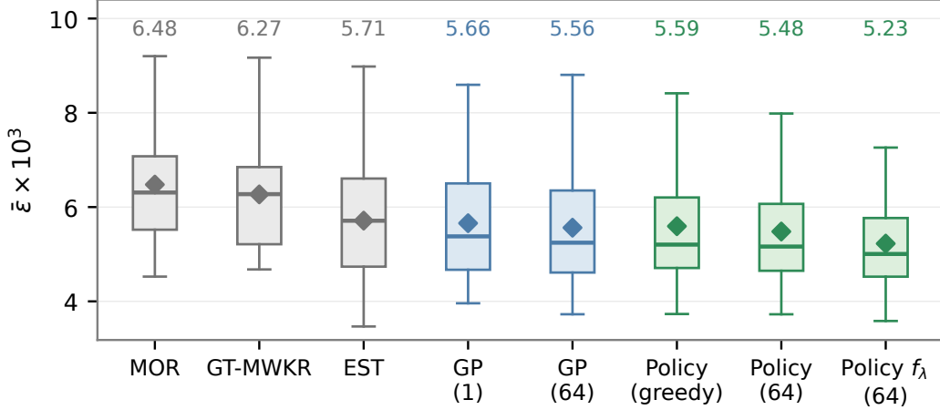
Figure 11: Executional robustness by method: \bar{\epsilon} \times 10^3 over the seventy benchmark instances; lower is a more faithful prediction. Boxes span the quartiles with whiskers at 1.5 IQR, and diamonds mark the means quoted in the text; the number in parentheses is the inference budget in constructed schedules.
