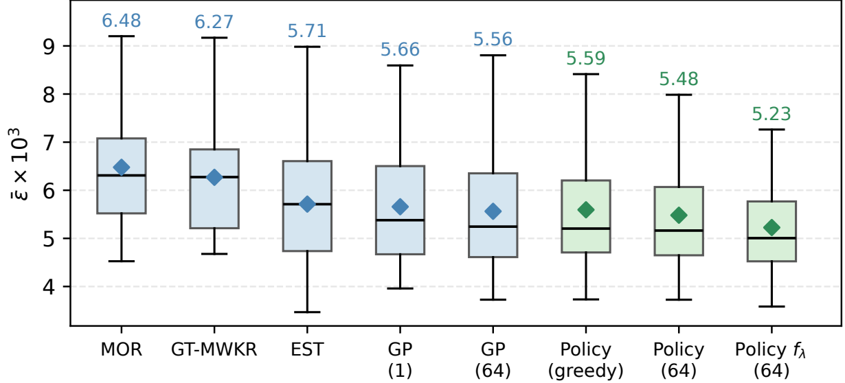
Figure 11: Executional robustness by method: \bar{\epsilon} \times 10^3 over the seventy benchmark instances; lower is a more faithful prediction. Boxes span the quartiles with whiskers at 1.5 IQR, and diamonds mark the means quoted in the text; the number in parentheses is the inference budget in constructed schedules.
