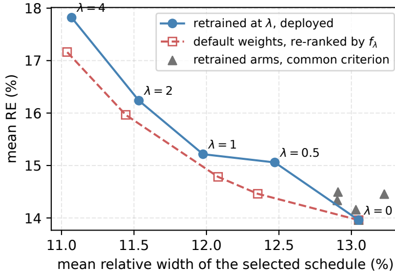
Figure 10: Mean relative width of the selected schedule against its mean RE, over the 60 (instance, seed) pools of each arm’s common rollout deposit, under three selection regimes.
