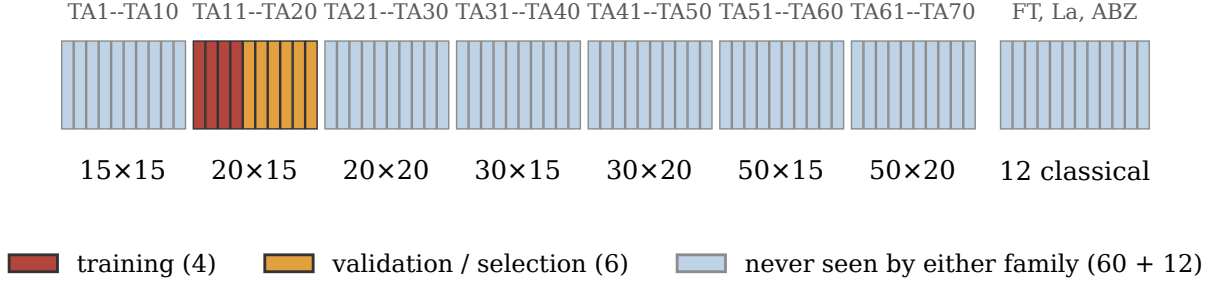
Figure 3: The data split. Both learners train on TA11–TA14 and take every design decision on TA15–TA20, all of the 20×15 class; the remaining sixty Taillard instances and the twelve classical ones are seen by neither family before evaluation.
