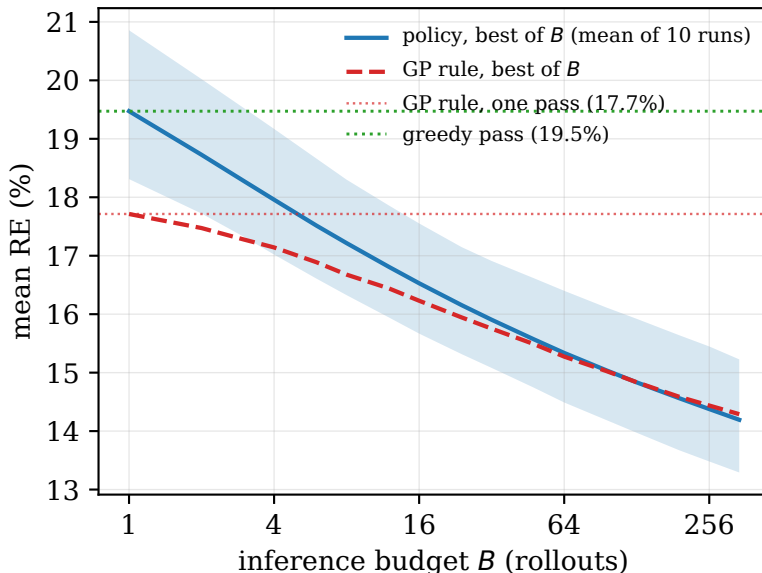
Figure 9: RE against the inference budget B on a base-2 logarithmic axis, for both learners under the same decoder: the schedule each retains from its deterministic pass plus B - 1 samples, kept by the criterion of Eq. (3) and averaged over the 70 instances. The policy curve is the mean over the ten training runs and the band spans the best and worst of them; the dotted line marks the rule’s single deterministic pass.
