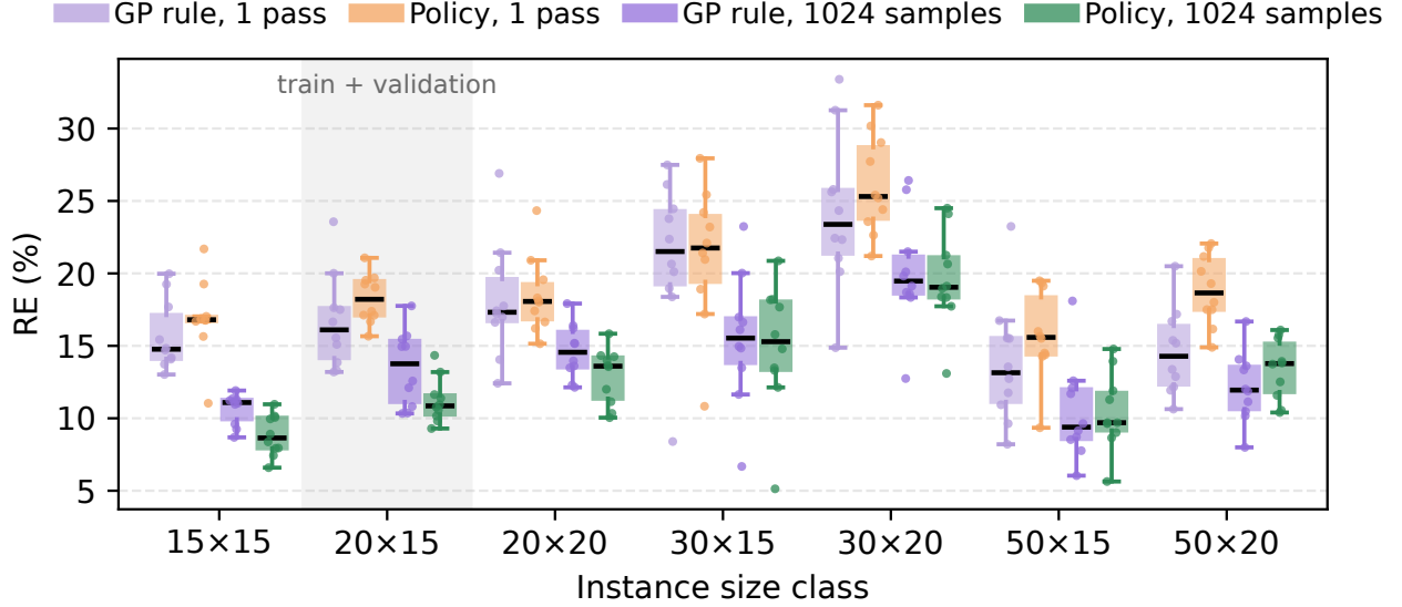
Figure 6: RE by size class over the 70 interval Taillard instances, the two learners paired at one pass and at 1024 samples. Boxes span the quartiles with whiskers at 1.5 IQR; every instance is overlaid as a point. The shaded 20 \times 15 class holds the training and validation instances.
