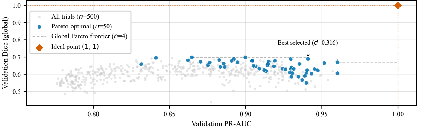
Fig. 2. Validation objective space across all 500 HPO trials (10 folds \times 50 MOTPE trials). Grey: evaluated; blue: Pareto-optimal; dashed: Pareto frontier. Red diamond: ideal point (1, 1); annotated point: selected configuration (distance d = 0.316 ).
