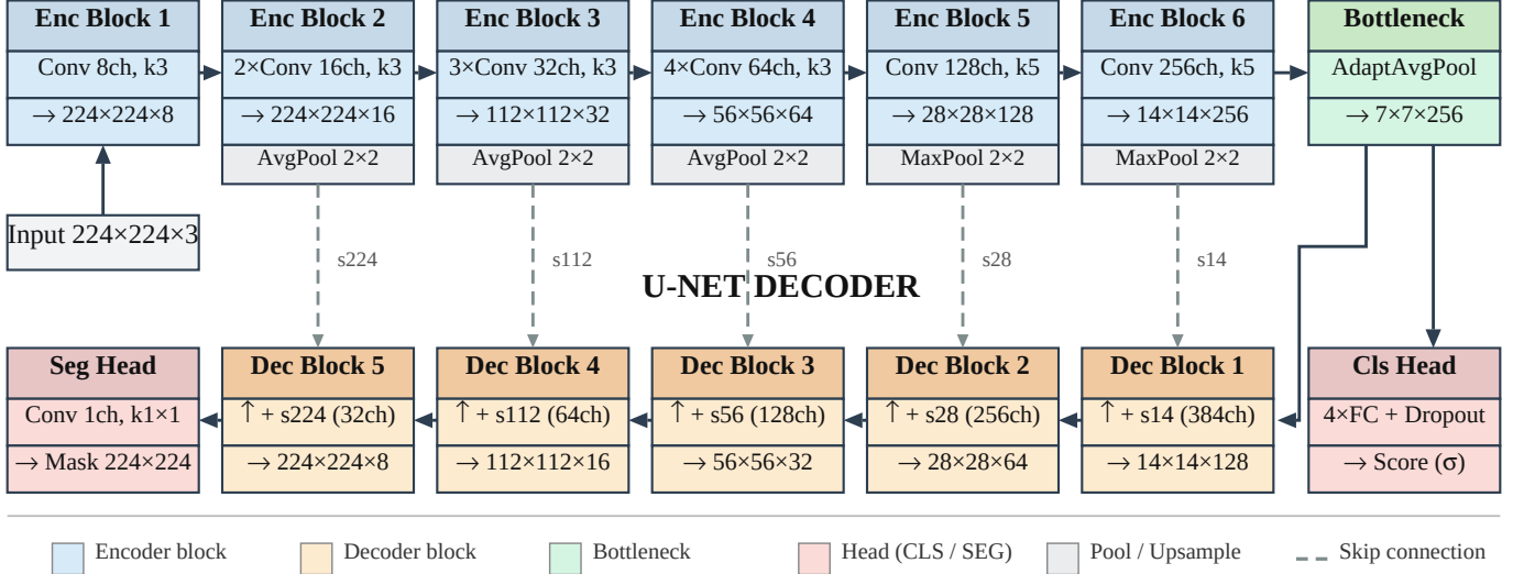
Fig. 1. DocVerify architecture. The encoder maps a 3 \times 224 \times 224 input to a 256 \times 7 \times 7 bottleneck through six convolutional blocks ( 8 \rightarrow 256 channels). The U-Net decoder reconstructs the forgery mask via skip connections; the classification head outputs a document-level tampered/genuine score.
