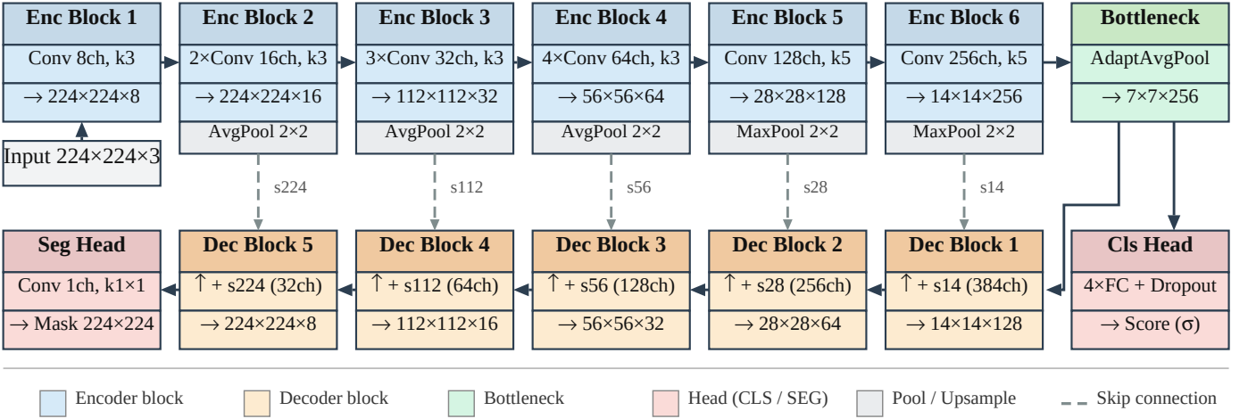
Fig. 1. DocVerify architecture. The encoder maps a 3 \times 224 \times 224 input to a 256 \times 7 \times 7 bottleneck through six convolutional blocks (8 → 256 channels). The U-Net decoder reconstructs the forgery mask via skip connections; the classification head outputs a document-level tampered/genuine score.
